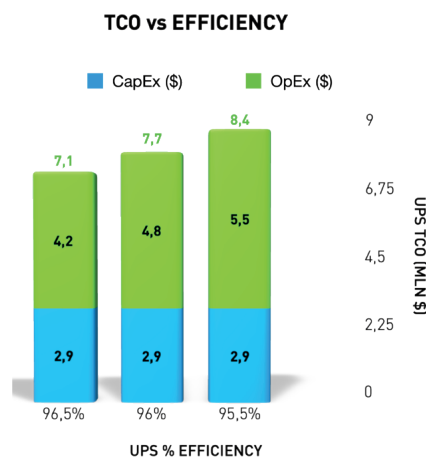
Correlation between TCO and efficiency
