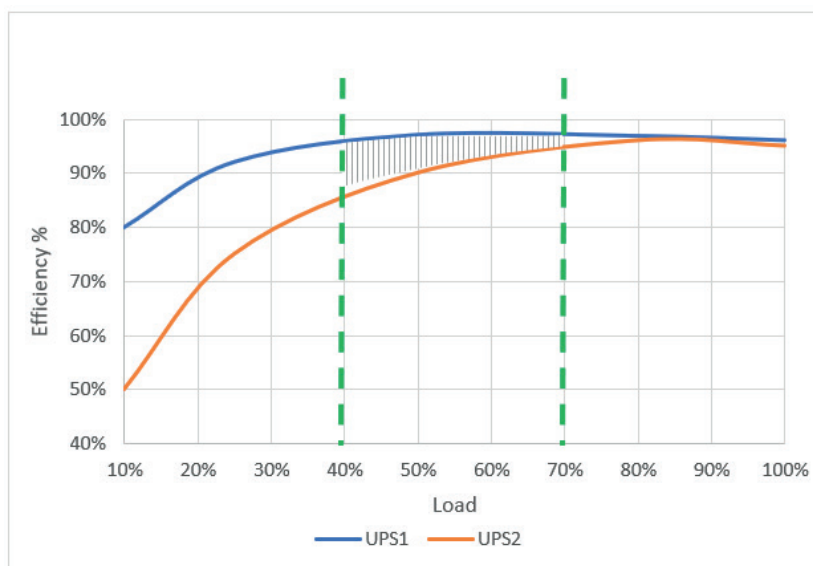
Legrand UPS' energy savings at low load percentages
