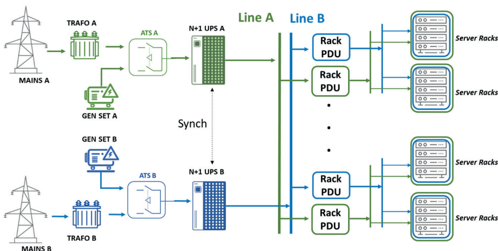
Compatibility with various configurations of the Electrical System
