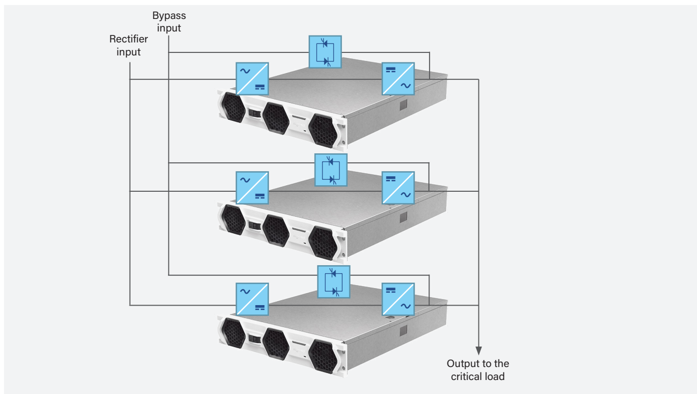
Figure 4: Modular UPS with N+X Redundancy
