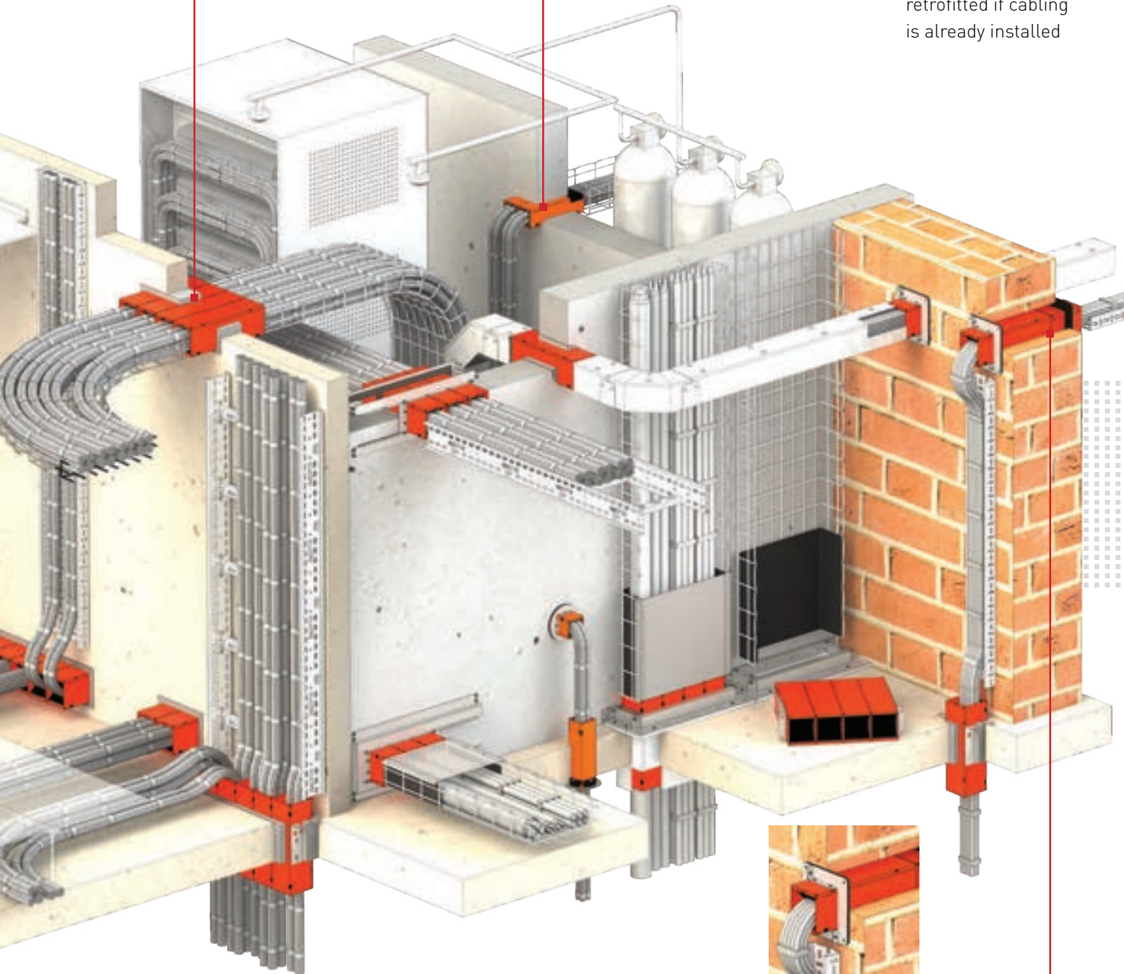
4 Extension pieces available for walls thicker than 250mm
